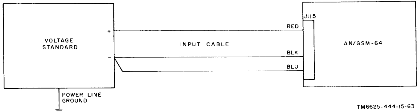
Figure 8-2. Standardization, ranging and polarity ( \pm offset).
