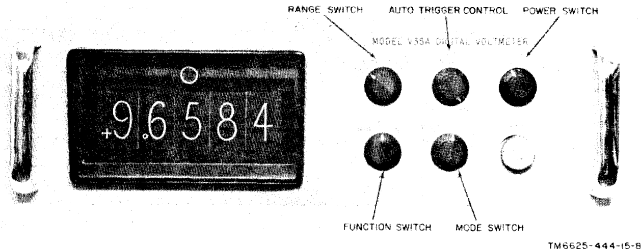
Figure 3- 1. Digital Voltmeter AN/GM-64 front panel controls.
