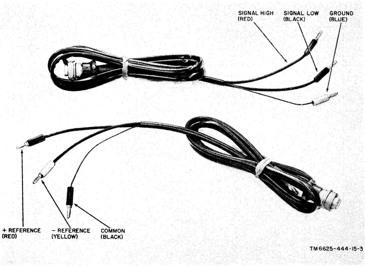
Figure 1-3. Signal input cable assembly CX-7495/GSM-64 (top), and External reference supply cable CX-7494/GSM-64 (bottom).
