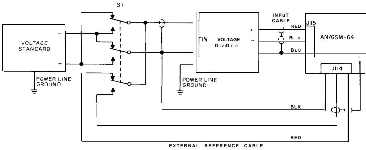
Figure 8-3. Dc voltage ratio test setup.
