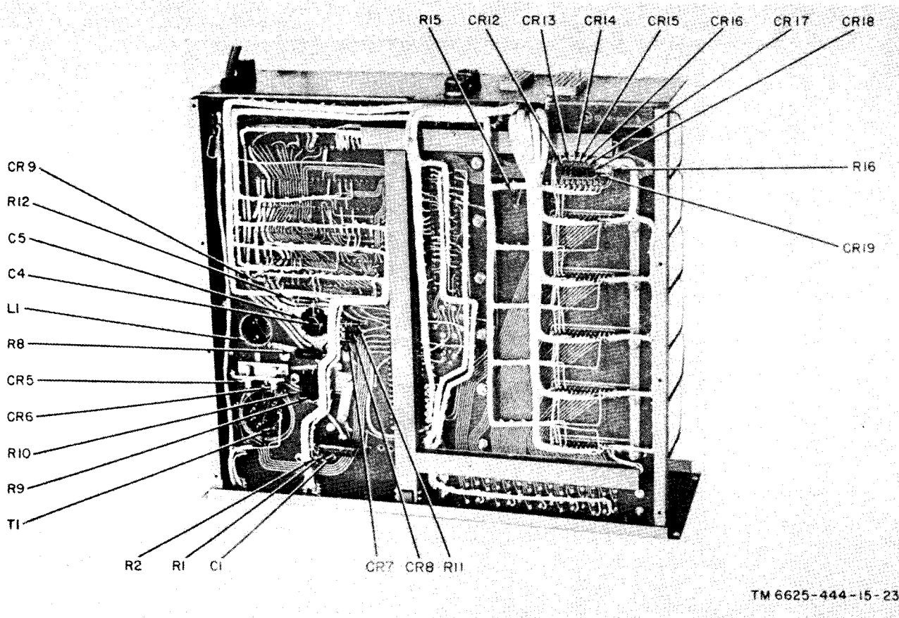
Figure 6-3. Digital voltmeter, serial number 11.3810 and up, bottom view.
