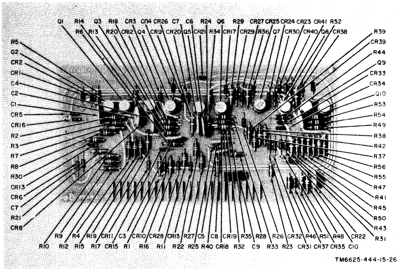
Figure 6-6. B board, parts identification.
