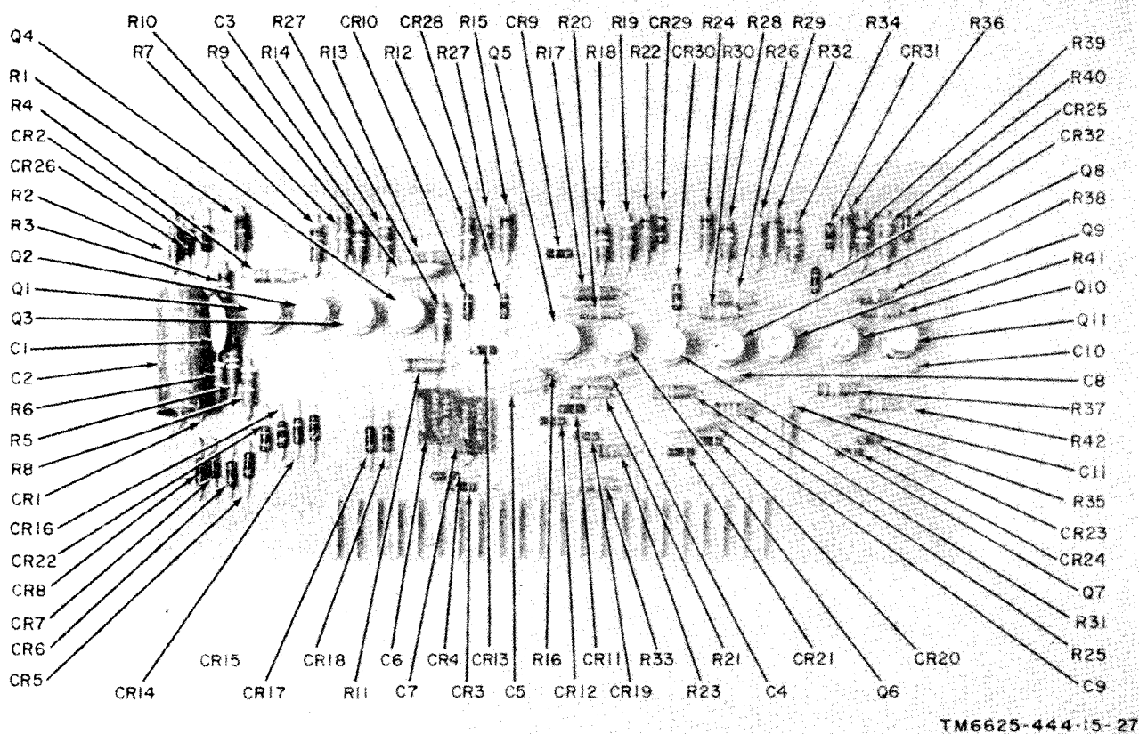
Figure 6-7. C board, parts identification.
