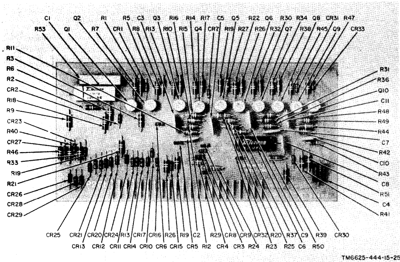
Figure 6-5 A board, parts identification
