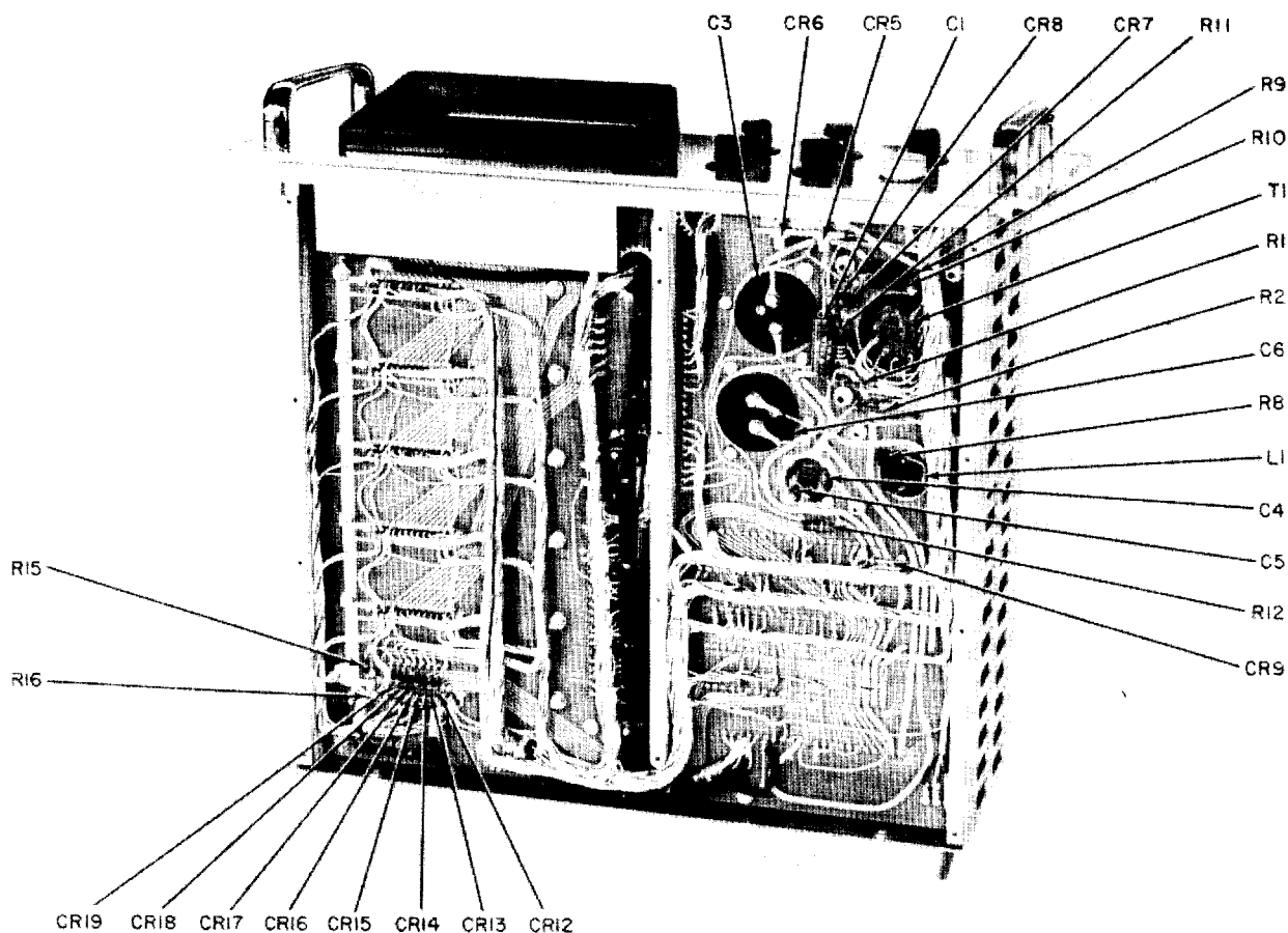
Figure 6-2. Digital voltmeter, up to serial number 11.3810, bottom view.
