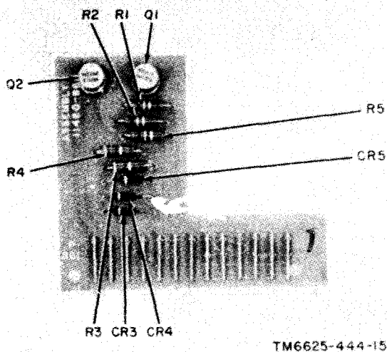
Figure 6-12. Decimal check board, parts identification.
