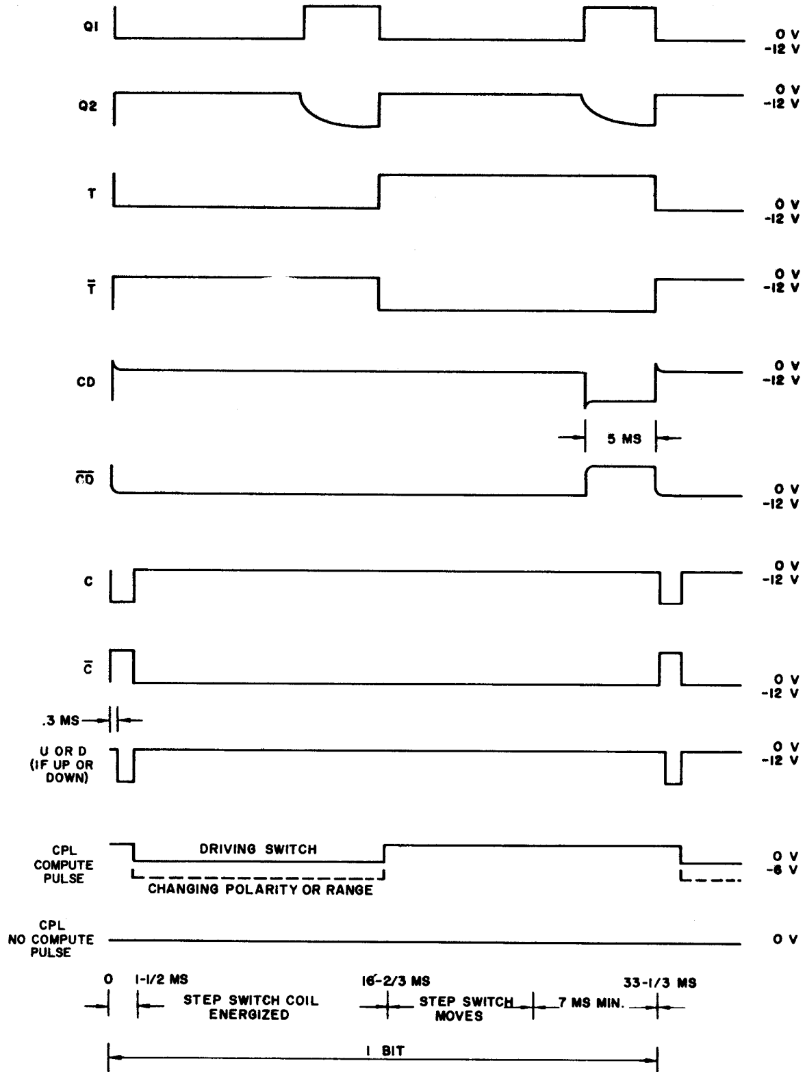
Figure 5-6. Timing chart.
