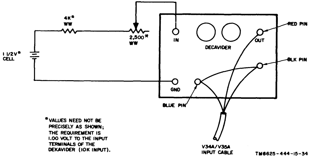
Figure 6-14. Troubleshooting test setup.
