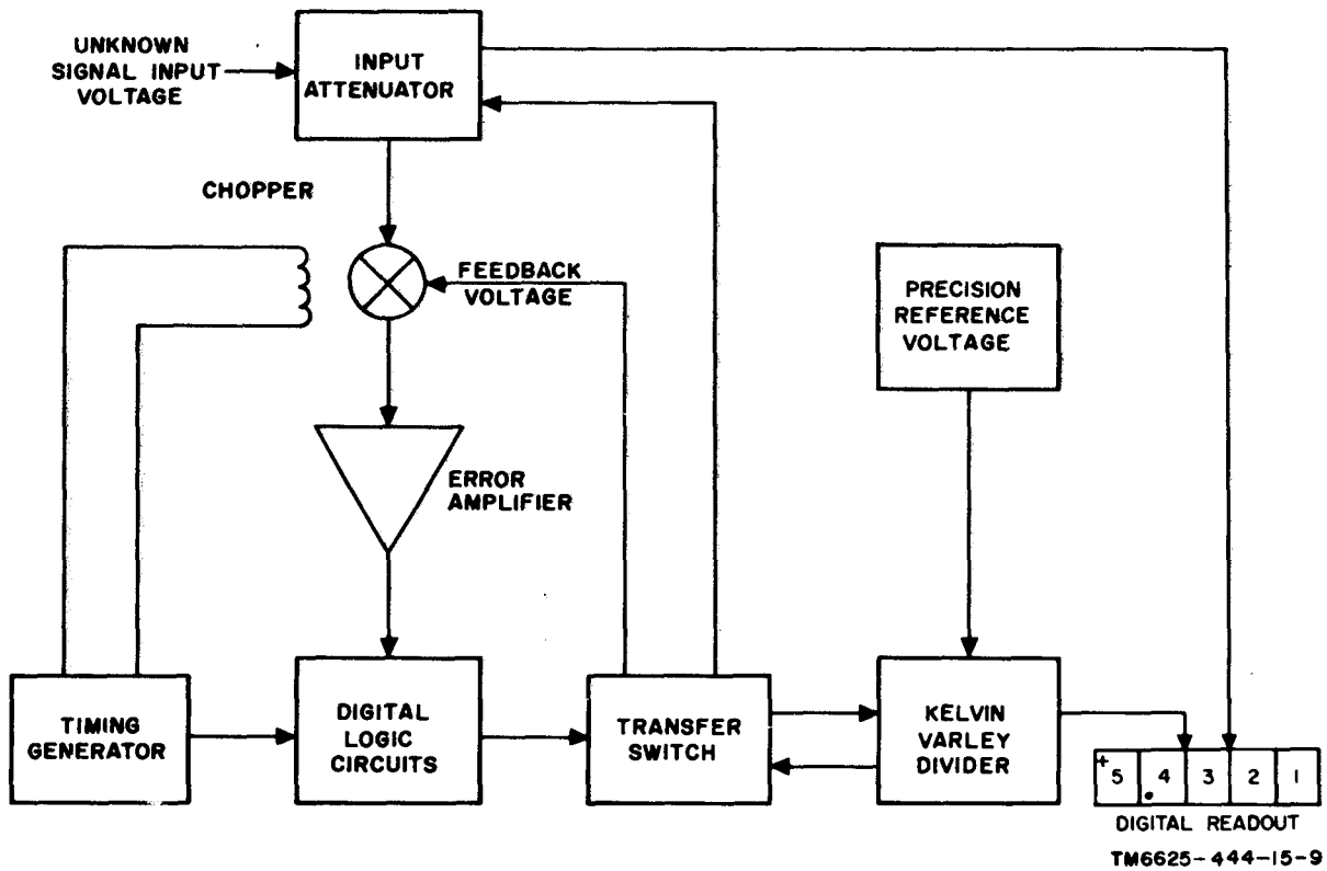
Figure 5-1. AN/GSM-64, block diagram.
