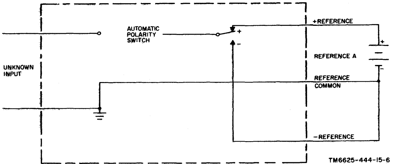
Figure 2-3. External reference supply connection to measure input voltages of single polarity.
