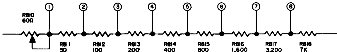
Figure 7-1. Jumper connections for 10-volt alignment resistors.
