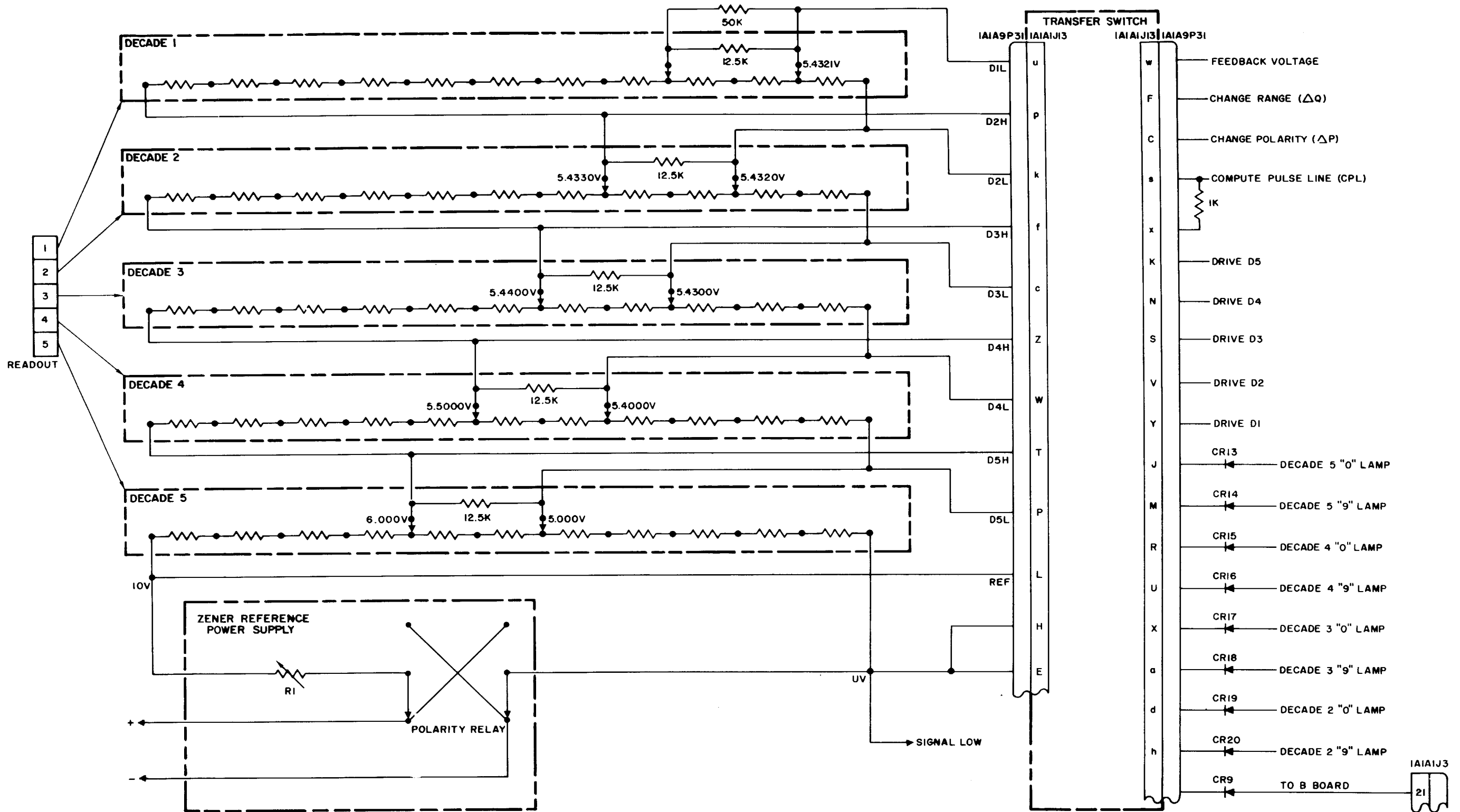
Figure 10-1. Stepping switch, Kelvin-Varley divider, and transfer switch circuitry.
