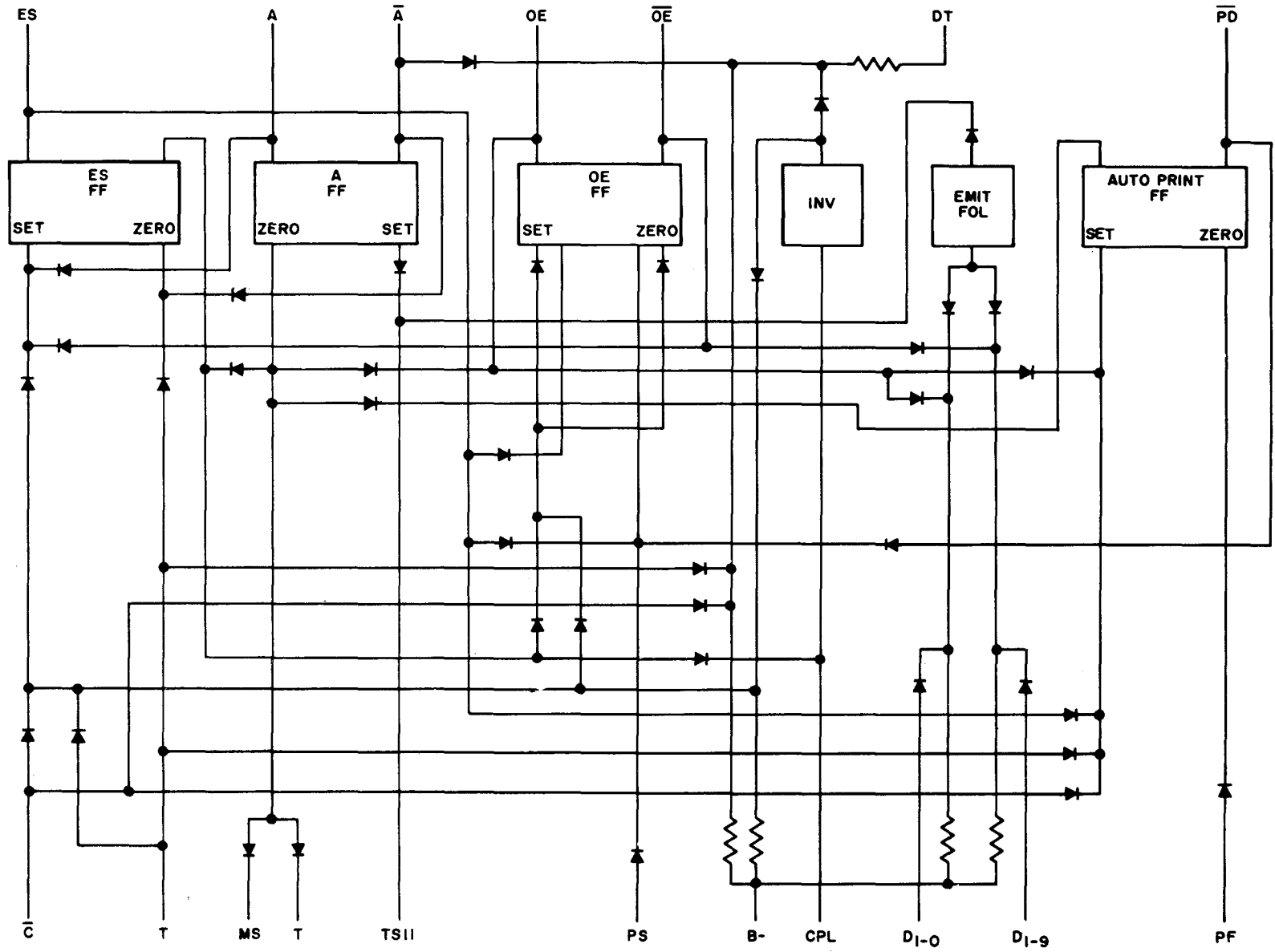
Figure 5-7. B board, block diagram.
