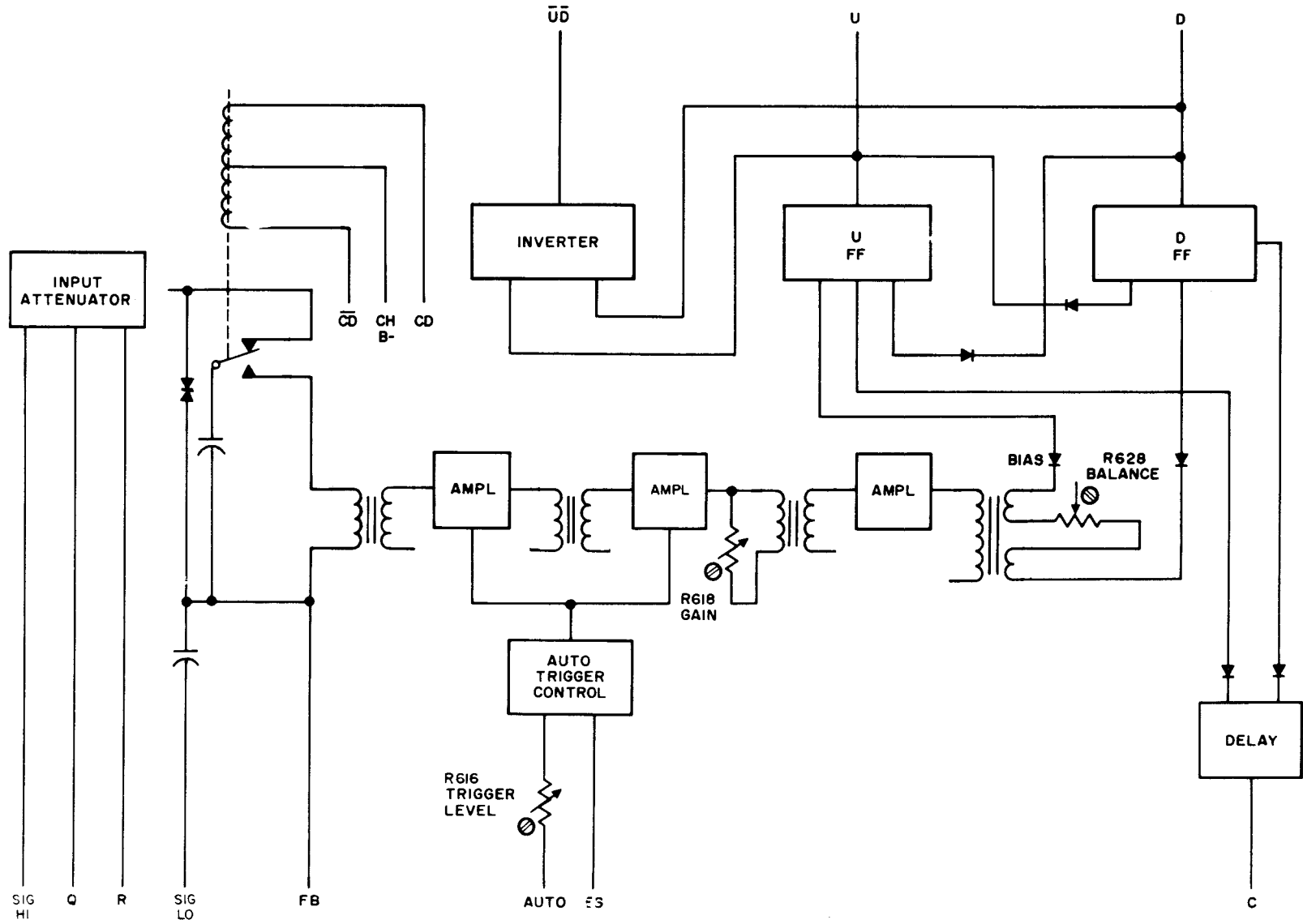
Figure 5-9. Error amplifier, block diagram.
