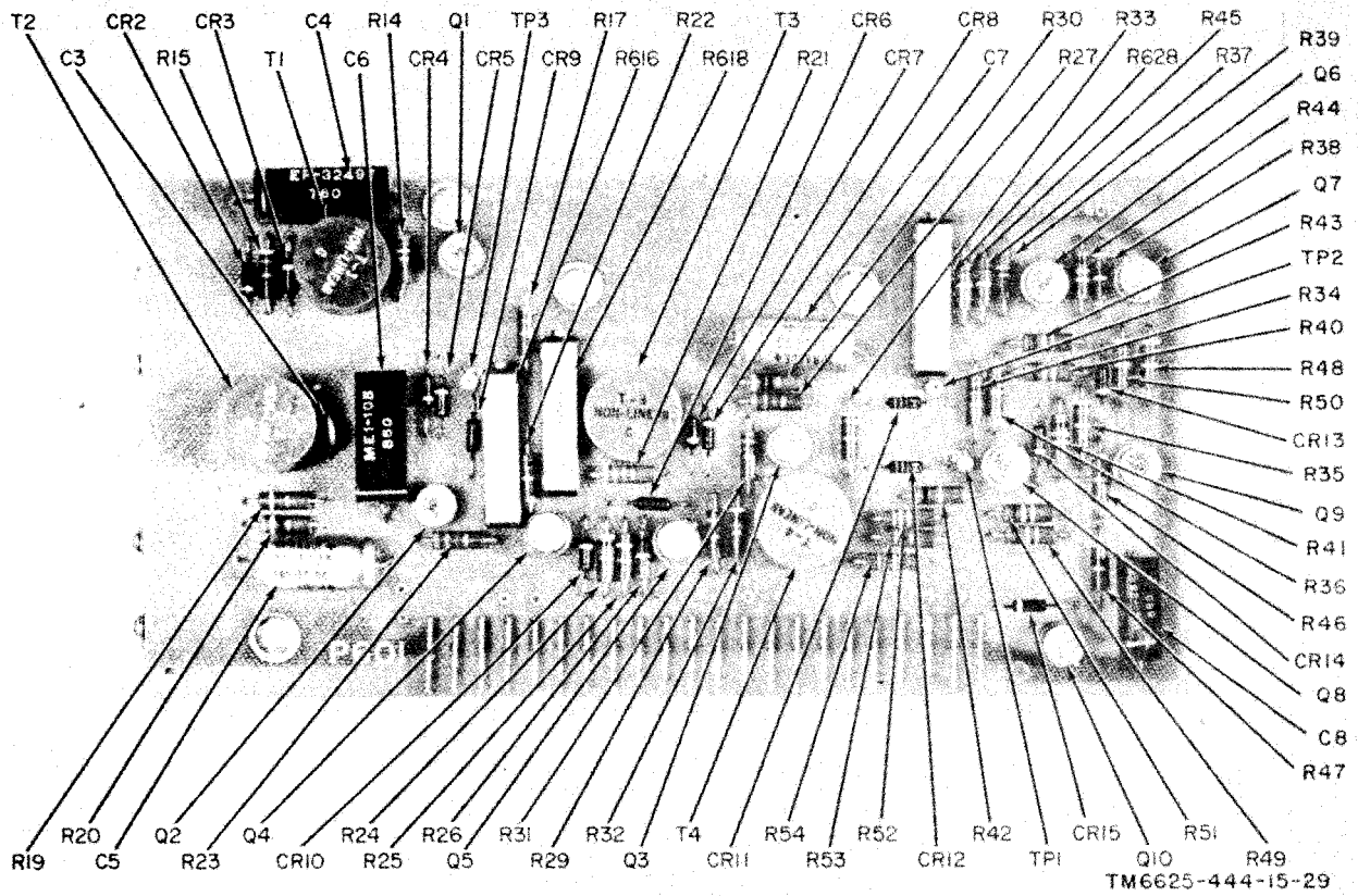
Figure 6-9. Amplifier board, parts identification.
