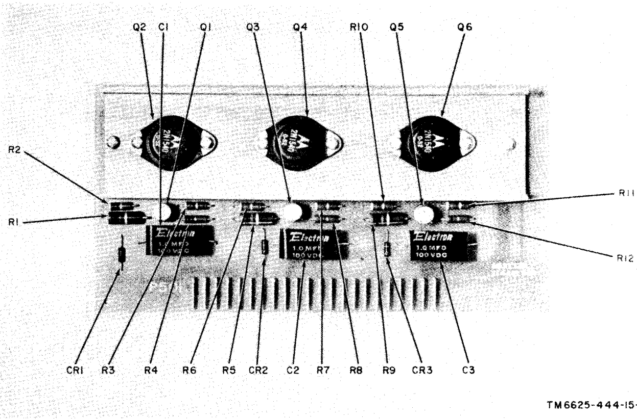
Figure 6-8. D board, parts identification.
