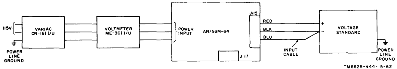
Figure 8-1. Operational test setup.
