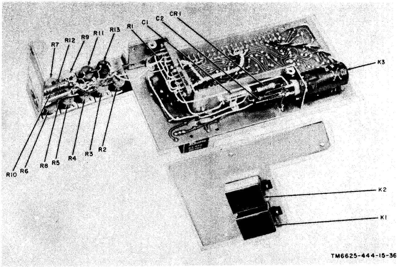
Figure 6-10. Amplifier board showing shield partially disassembled.
