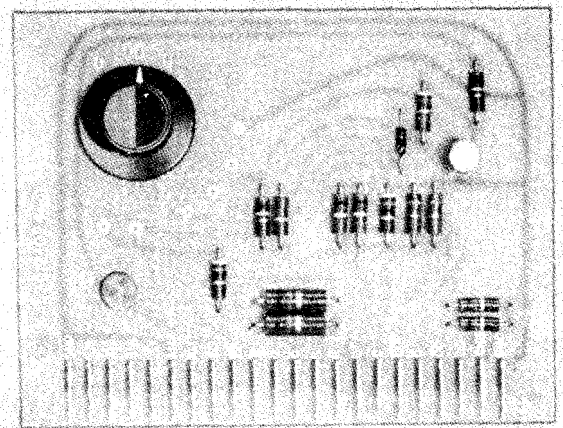
Figure 6-13. Dummy amplifier board.
