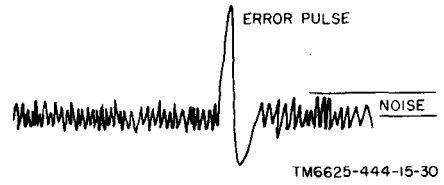
Figure 6-16. Amplifier output waveform.
