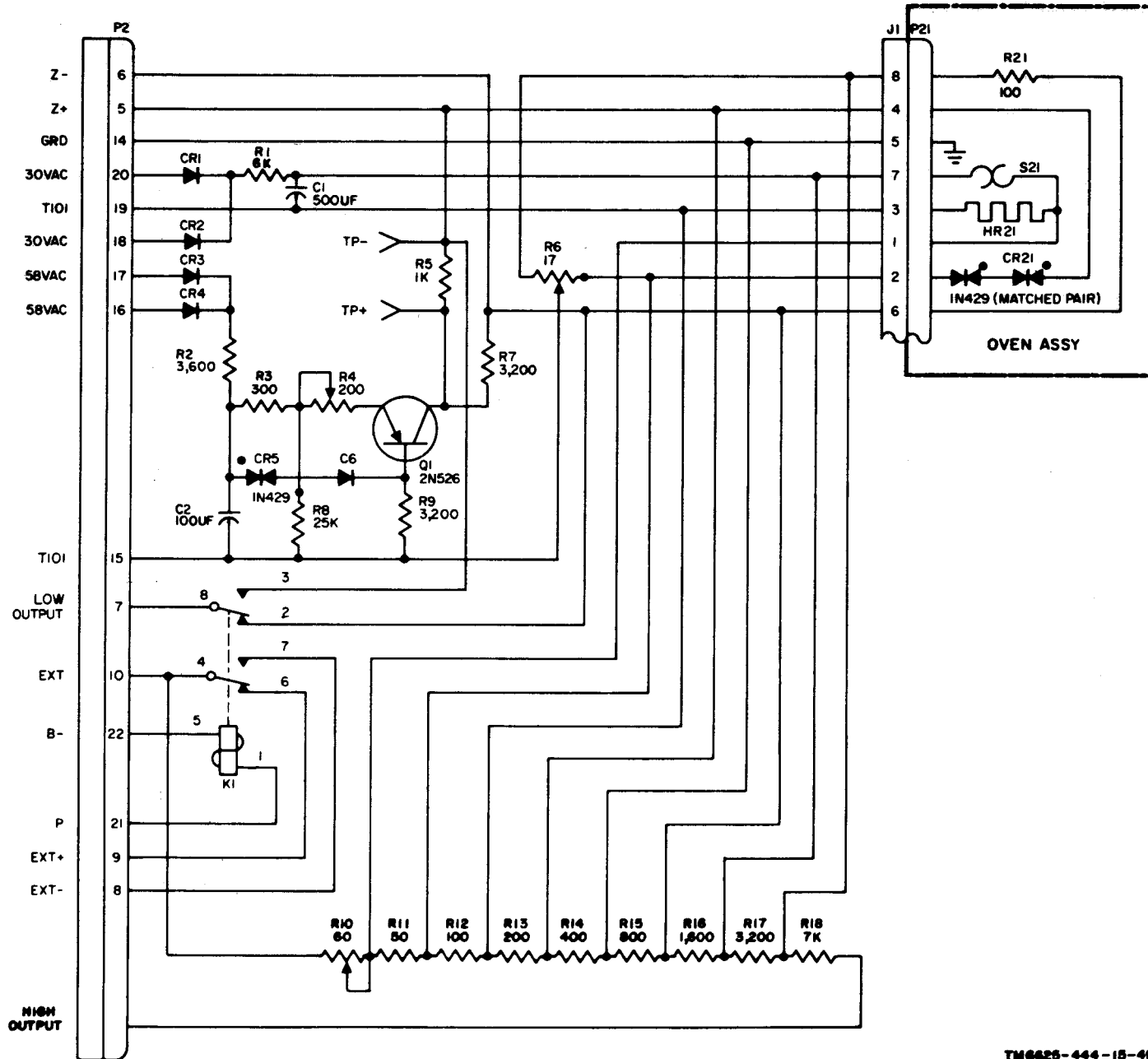
Figure 6-20. Zener supply assembly, schematic diagram.
