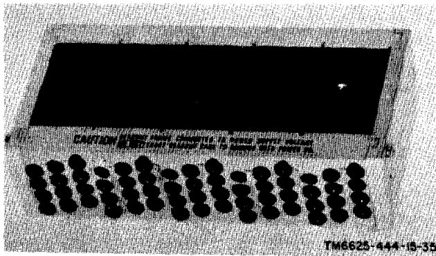
Figure 6-15. Front view of readout showing bulbs correctly positioned.
